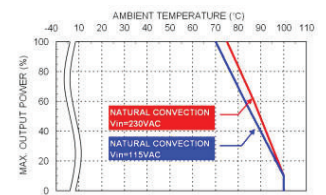
Derating Curve vs. Ambient Temperature KUI30-xxB xx=12, 15, 24, 28, 36, 48, 53 Connector Option: (-M, -T, -D)
